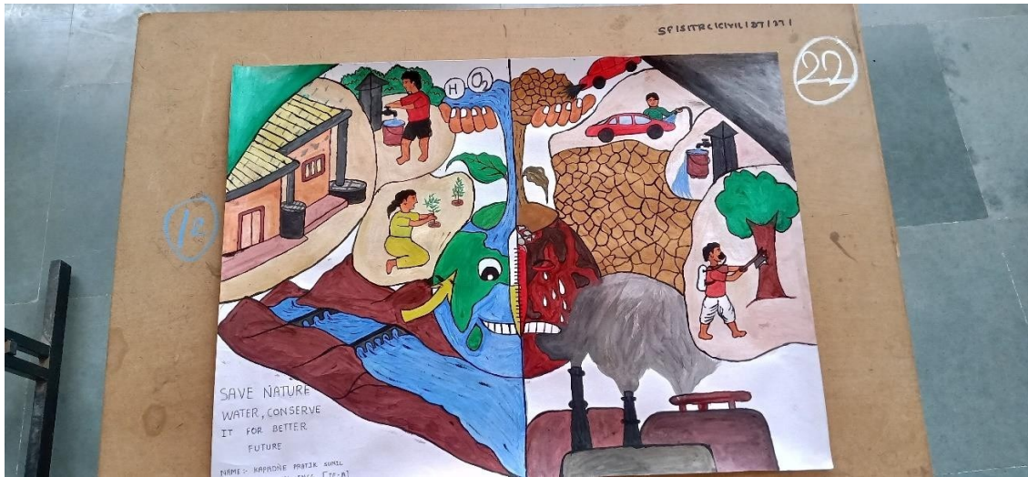
2 nd Rank
